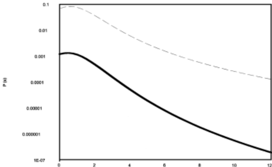
FIG. 1. Transition rate P as a function of the distance s from the metal surface for a proton scattered from aluminum surface (solid curve for the case when a bulk plasmon is excited while the dashed curve represents the case when a surface plasmon is excited).
